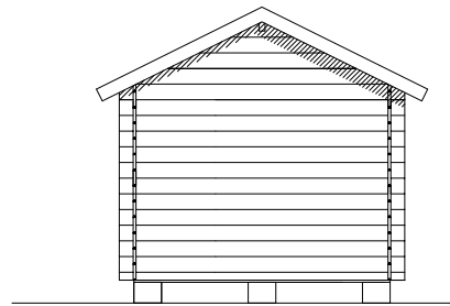
Gavelsida
